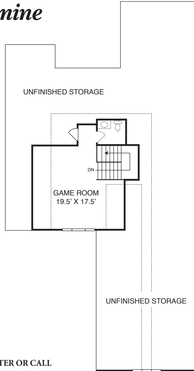
SECOND FLOOR
